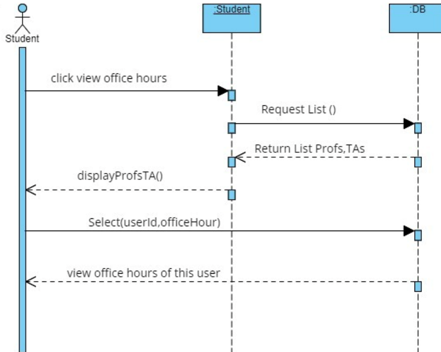
Figure 9. View Office Hours sequence Diagram (Ecom 2023)
