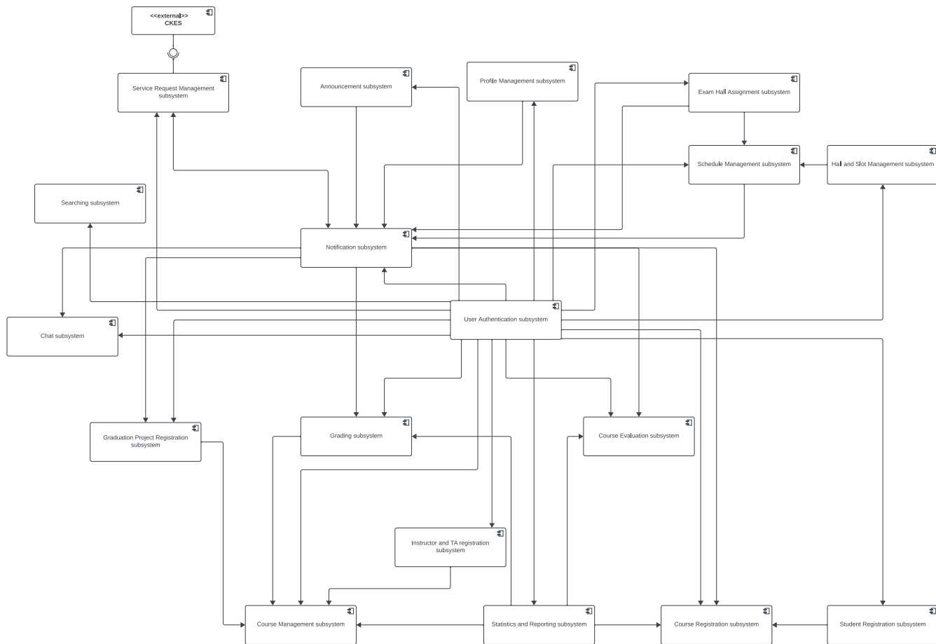
Figure 6. Component Diagram
