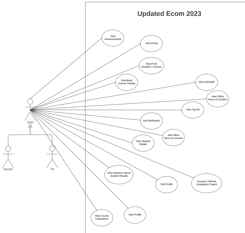
Figure 2. Use Case Diagram for Professor and TA (Ecom 2023)
