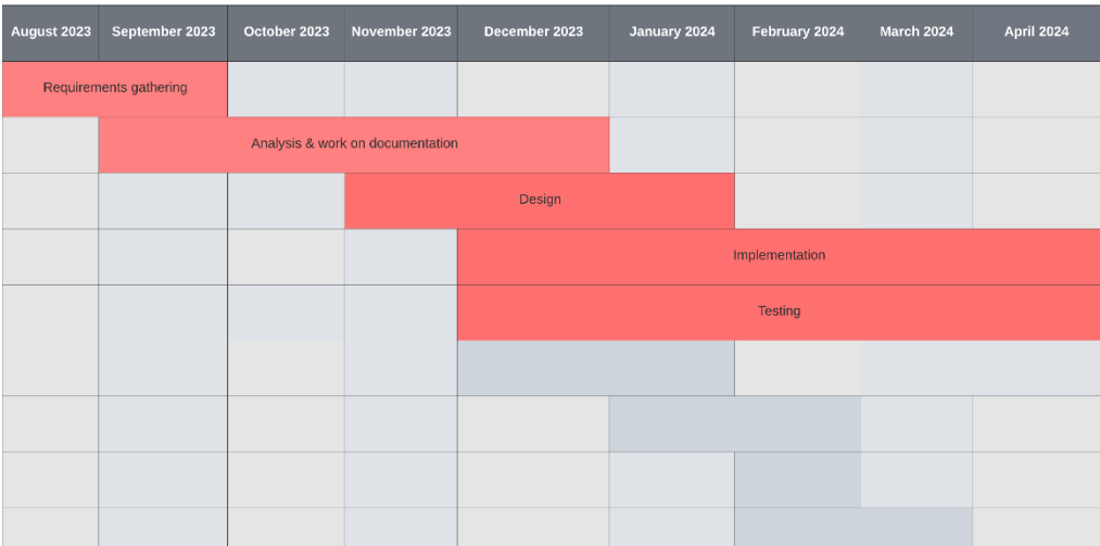
Figure 1. Gantt Chart
