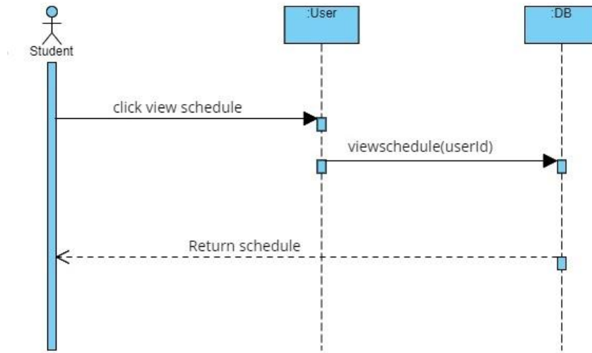
Figure 10. View Schedule Sequence Diagram (Ecom 2023)
