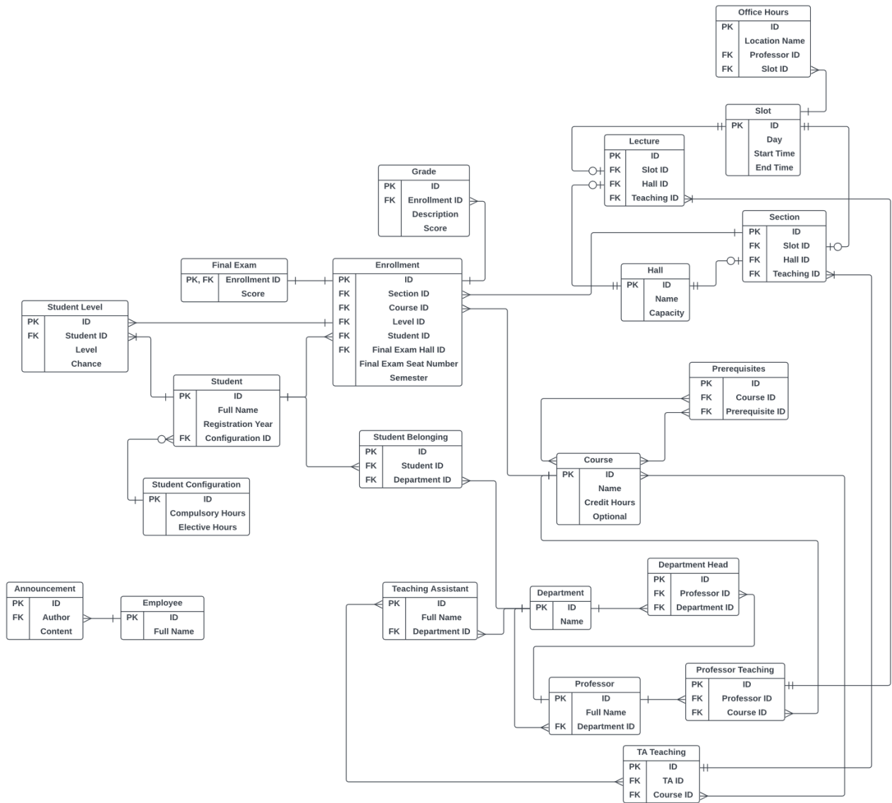
Figure 5. ERD
