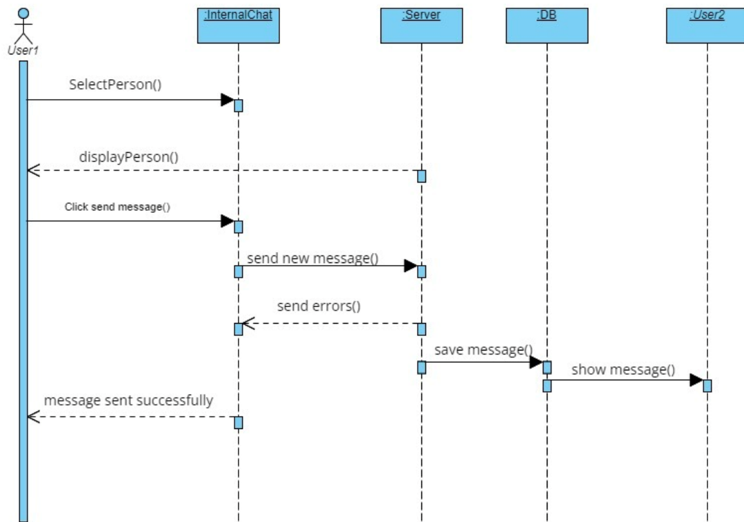
Figure 8. Internal Chat (Ecom 2023)
