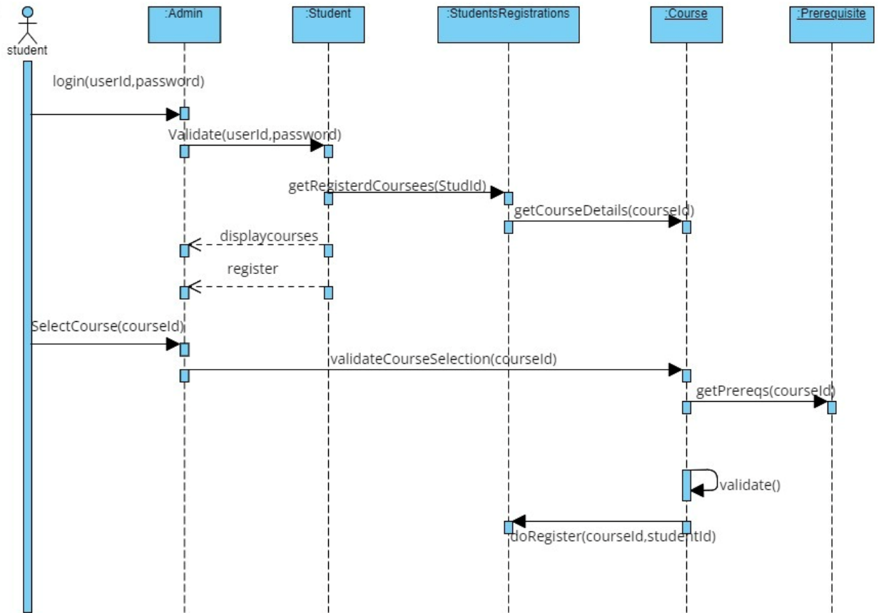
Figure 7. Register Course Sequence Diagram (Ecom 2023)
