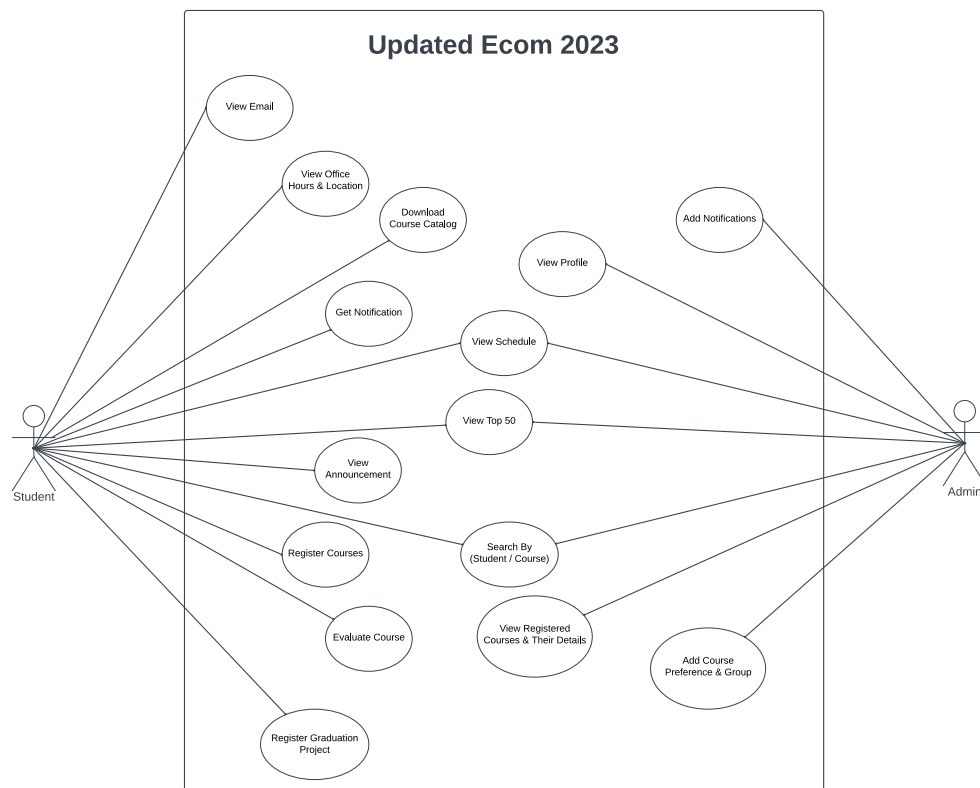
Figure 3. Use Case Diagram for Student and Admin (Ecom 2023)
